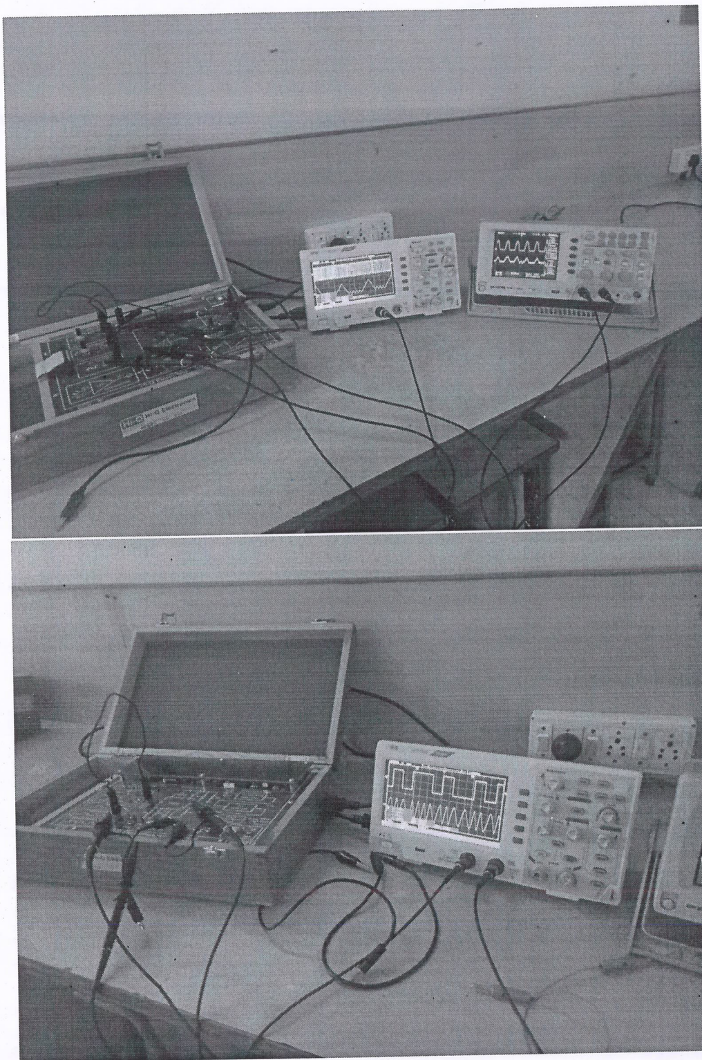
Analog and Digital Filter Design Exploring Signal Filtering Using Digital Storage Oscilloscope
