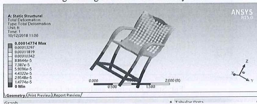
Fig: Deformation of chair in static structural
