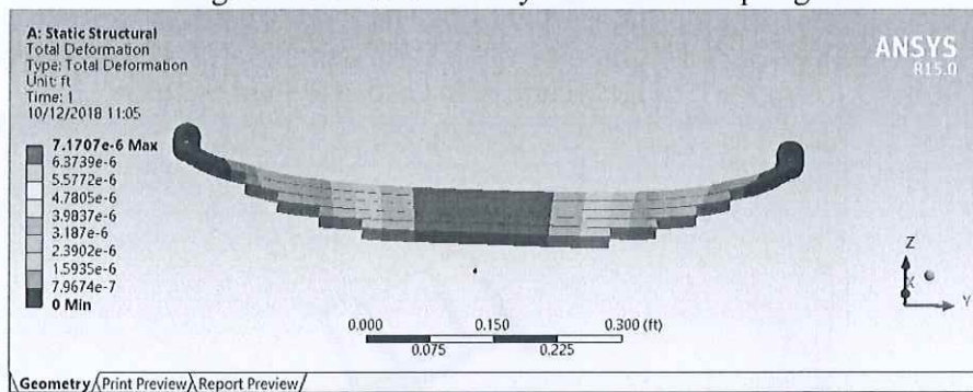
Fig: Static Structural analysis on Leaf Spring
