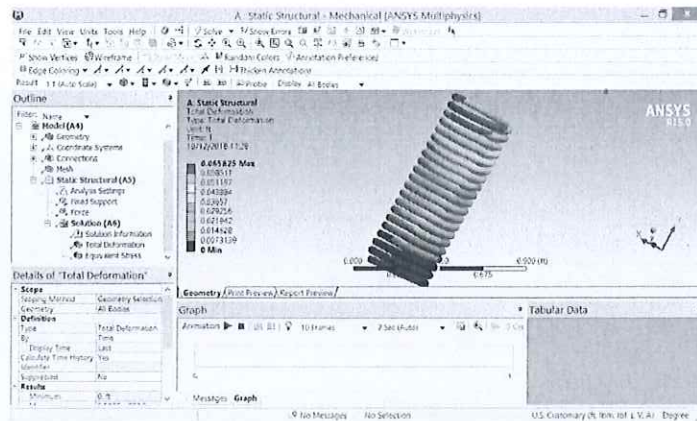
Fig: Static Structural analysis on Helical Spring
