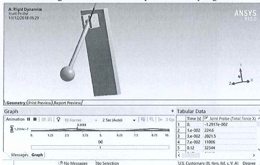
Fig: Oscillation of Pendulum in rigid dynamics
